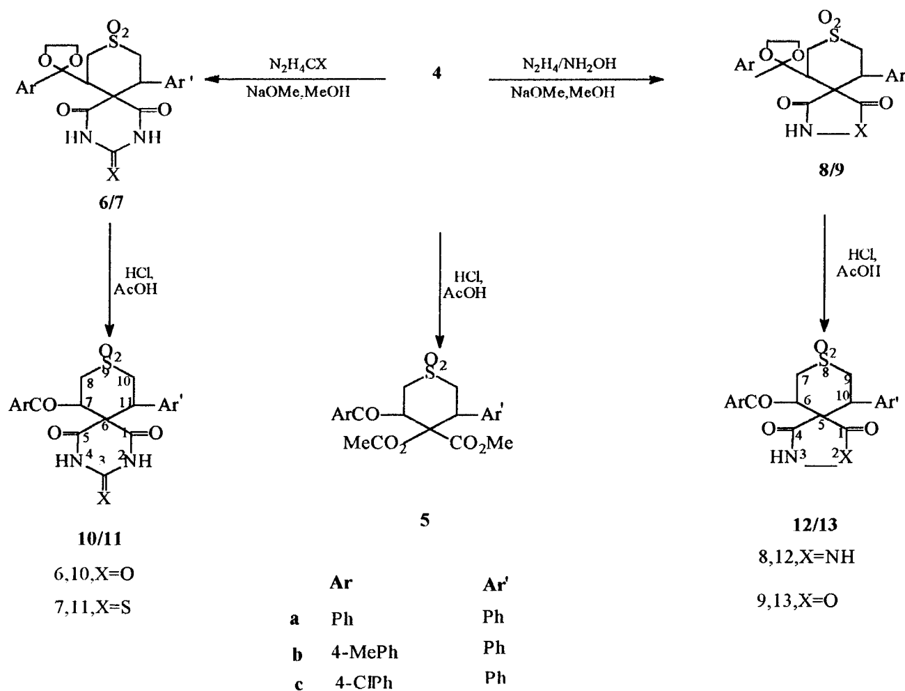
SCHEME 2
